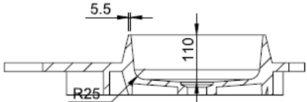
SECTION AF-AF
